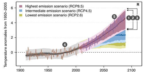
FIGURE 2: SIMULATED HISTORICAL AND PROJECTED TEMPERATURE (°C) TIME-SERIES FOR THE RANGELANDS CLUSTER, SHOWN AS DIFFERENCES FROM THE 1950–2005 AVERAGE. (SEE EXPLANATION BELOW).
