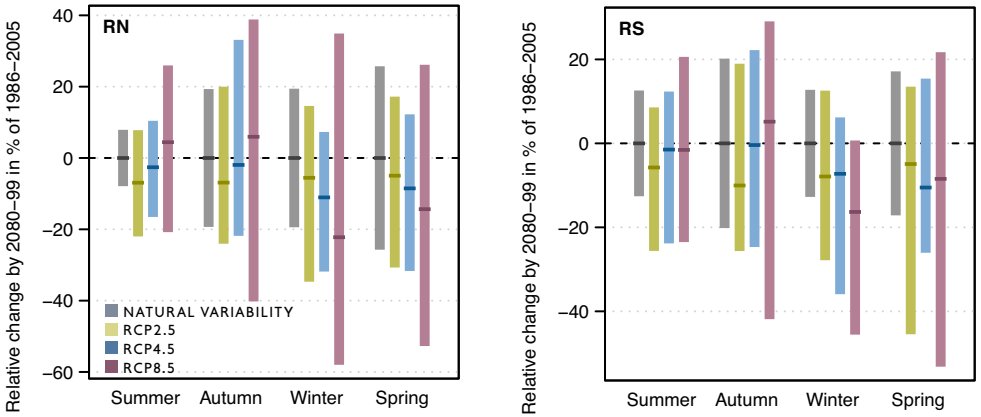
FIGURE 3: PROJECTED RAINFALL DIFFERENCES (PER CENT) FOR THREE RCPs FOR THE RANGELANDS SUB-CLUSTERS FOR 20 YEARS CENTRED ON 2090 COMPARED TO 1986–2005. BARS INDICATE THE 10TH TO 90TH PERCENTILE RANGE OF MODEL RESULTS. THE HORIZONTAL LINE INDICATES THE MEDIAN.
