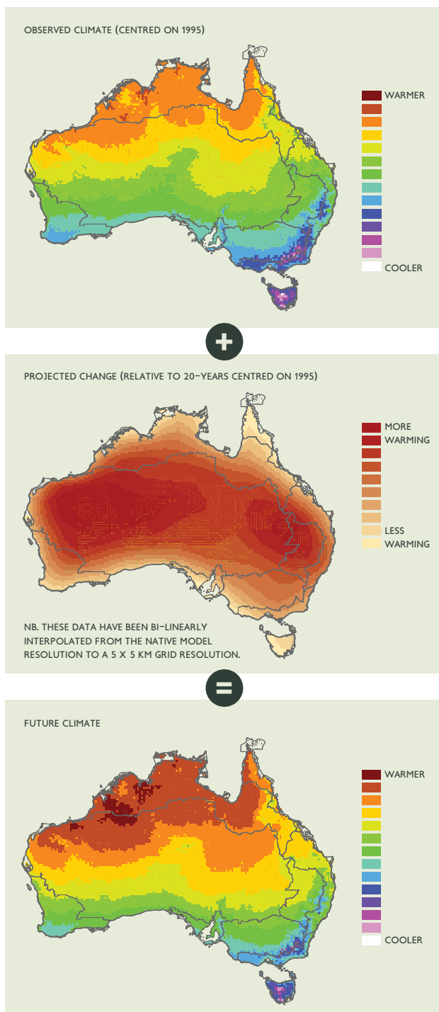
FIGURE 5: DELTA CHANGE METHOD FOR CALCULATING APPLICATION-READY FUTURE CLIMATE DATA.
