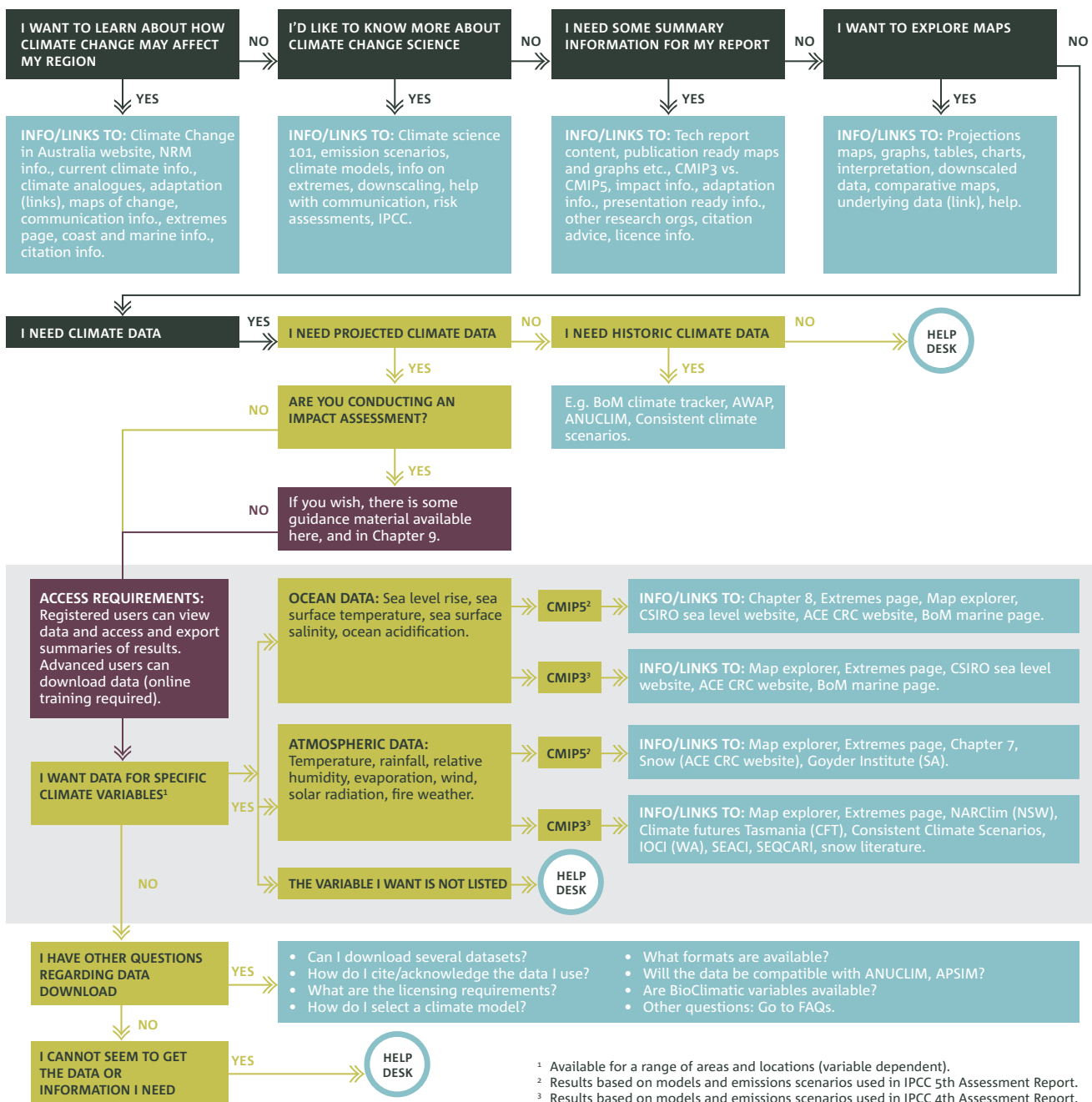
FIGURE 7: DECISION TREE AVAILABLE ON THE WEBSITE, WITHIN WHICH THE MAP EXPLORER PROVIDES A PATHWAY TO THE DOWNLOADABLE DATA PROVIDED FOR THE NRM PROJECT. PALE GREY BOX INDICATES REGISTRATION REQUIREMENT FOR ACCESS TO DATA AND INFORMATION.
