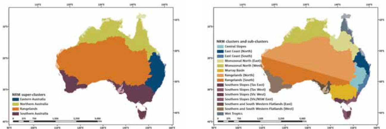
FIGURE 3: NRM SUPER-CLUSTERS (LEFT), CLUSTERS AND SUB-CLUSTERS (RIGHT).
