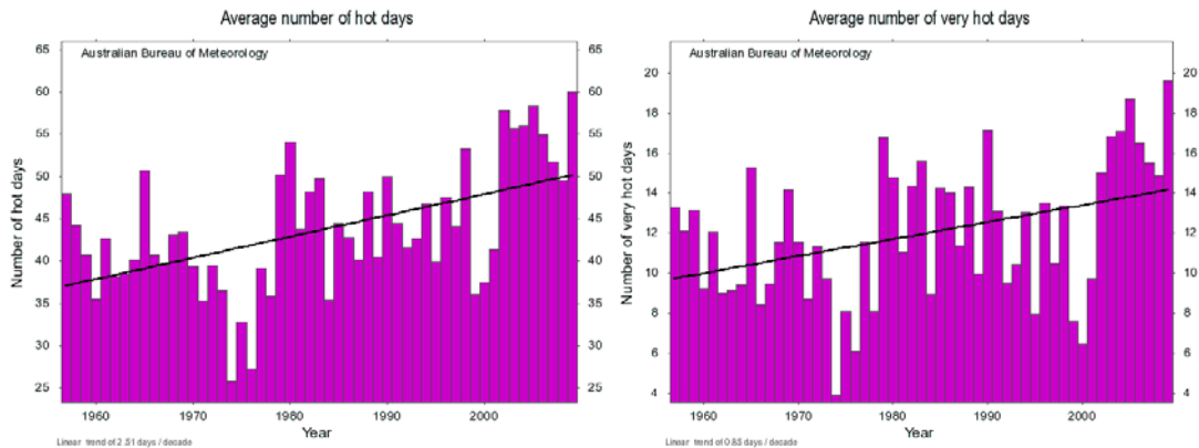
Figure 3. Australian-average annual temperature number of hot days (over 35°C) and very hot days (over 40°C) from 1957-2009. Source: Australian Bureau of Meteorology.
