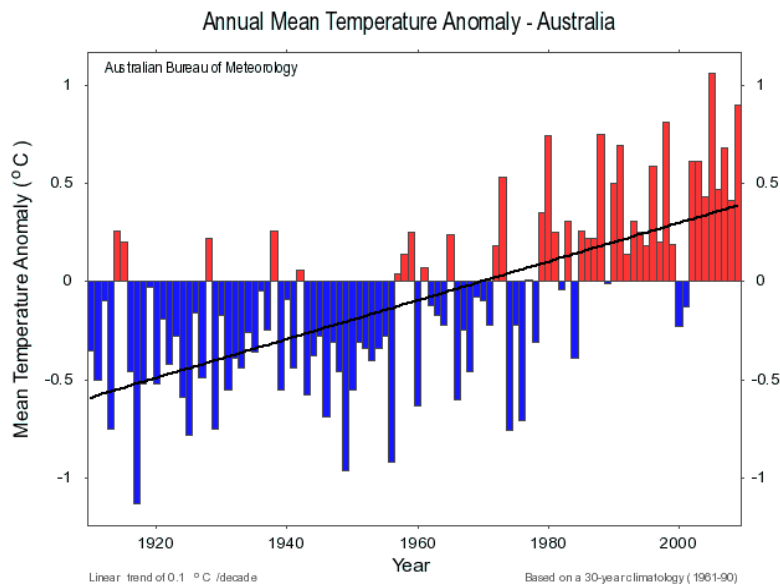
Figure 2. Australian-average annual temperature anomalies for 1910-2009 relative to the average for the 1961-1990 period. Source: Australian Bureau of Meteorology.
