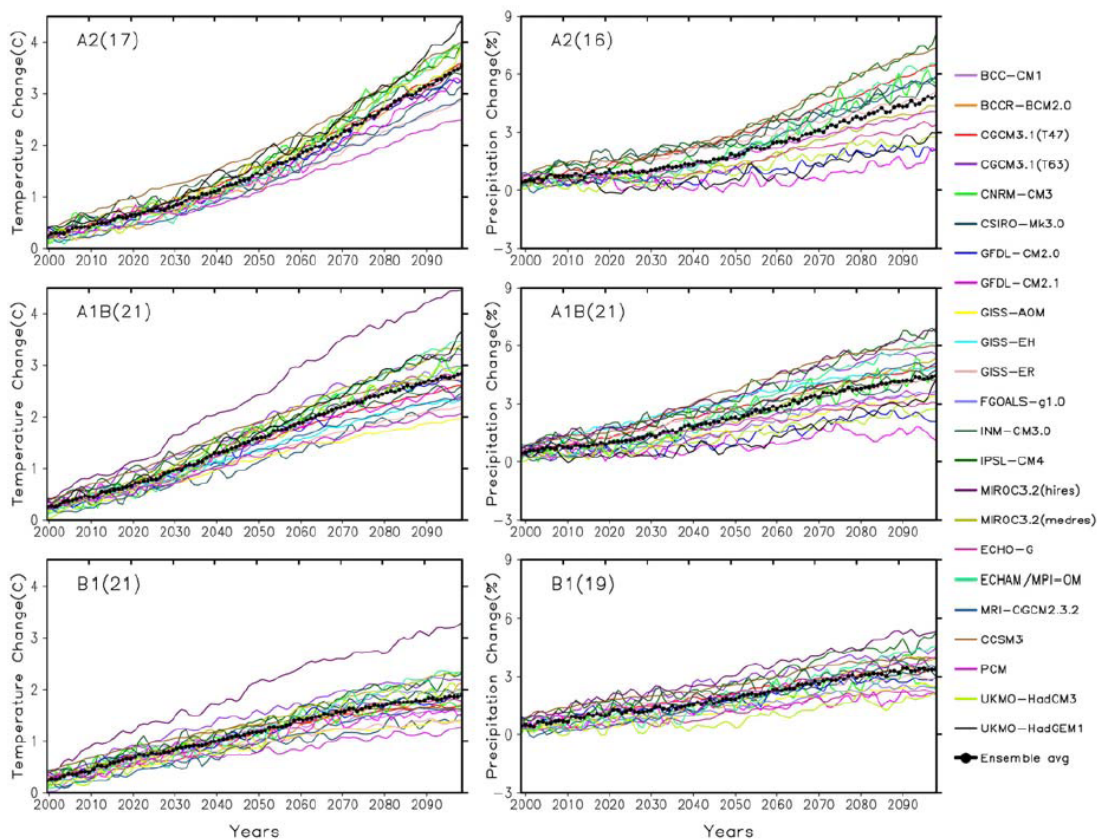
Figure 5: Global average change in temperature and precipitation from 23 global climate models during the 21 st century, relative to 1980-1999, for three emission scenarios (A2, A1B and B1). Source: IPCC (2007) Figure 10.5.
