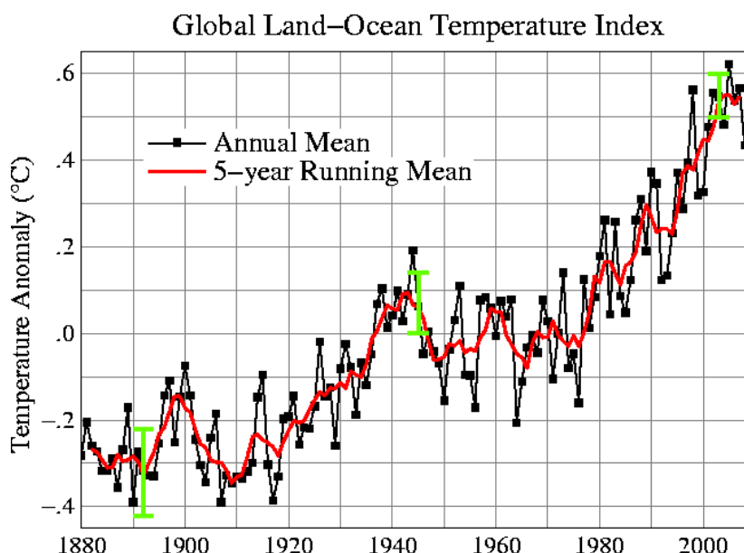
Figure 1: global mean land-ocean temperature anomalies, 1880 to present, relative to the base period 1951-1980. The dotted black line is the annual mean and the solid red line is the five-year mean. The green bars show uncertainty estimates. The warmest year is 2005 and the second-warmest is 2009. Source: http://data.giss.nasa.gov/gistemp/graphs .
