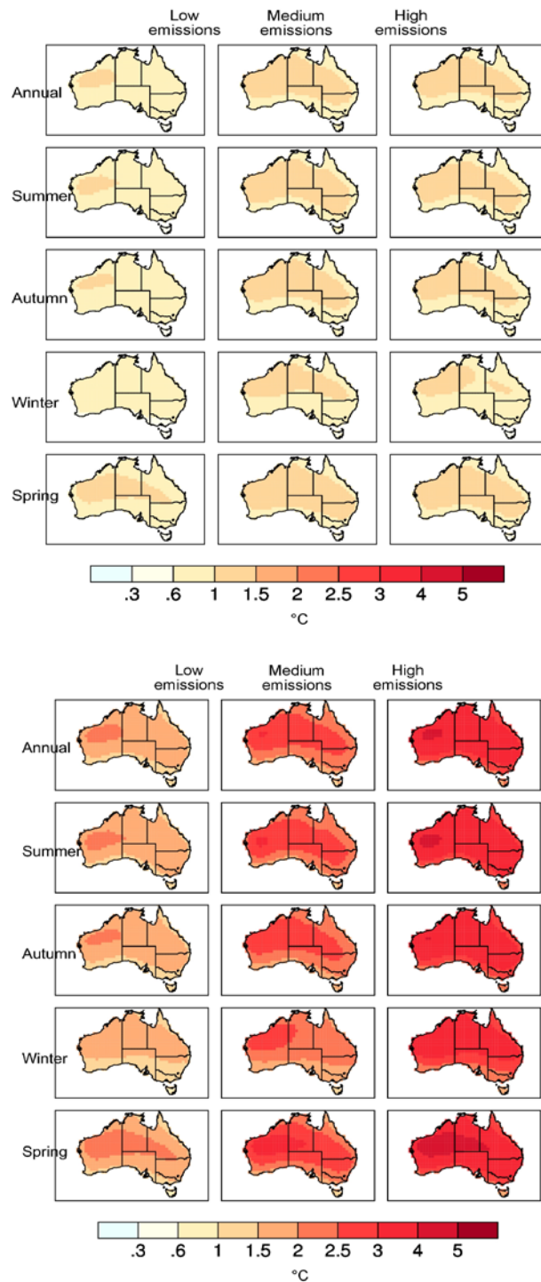
Figure 6: 50 th percentile changes in annual and seasonal mean temperature for 2030 (upper panel) and 2070 (lower panel), relative to 1980-1999, for low (B1), medium (A1B) and high (A1FI) emission scenarios. Source: http://www.climatechangeinaustralia.gov.au/
