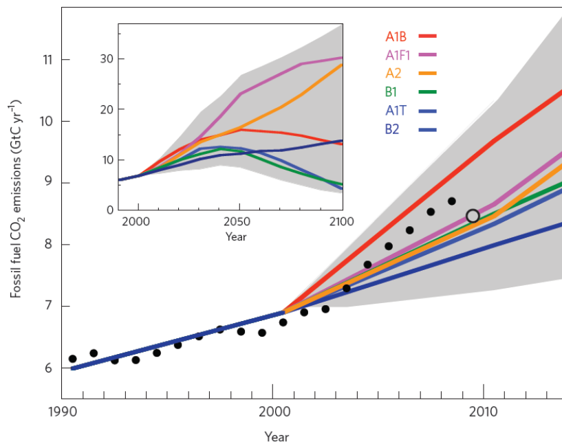
Figure 4. CO 2 emissions (Gt/year) from 1990-2009 (black dots) compared with IPCC scenarios (grey shading shows the full range, while coloured lines show 6 “marker” scenarios). The open circle shows an estimate for 2009 which includes the effect of the global financial crisis. The inset plot shows IPCC emission scenarios from 1990-2100. Source: Manning et al (2010).
