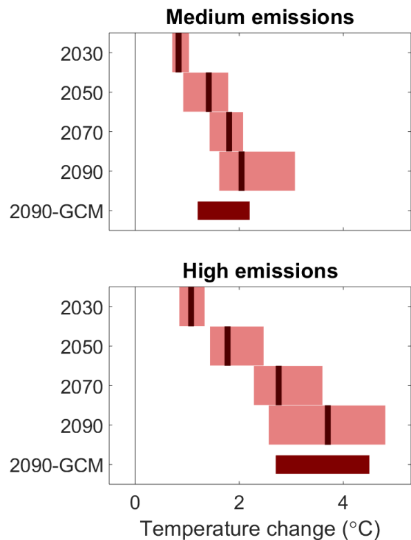
Figure 1. Projected changes in annual mean temperature for medium emissions (top) and high emissions (bottom). Light red bars: results from the full range of new downscaled modelling. Dark vertical line: median. Dark red bar: 2090s results from the most recent generation of global climate models for comparison.
